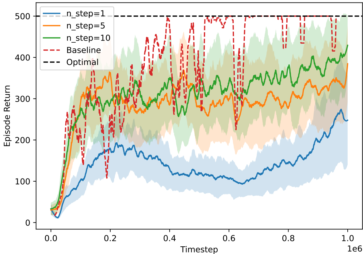
A2C estimation depth n
